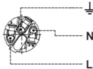
PowerCon connector configuration
