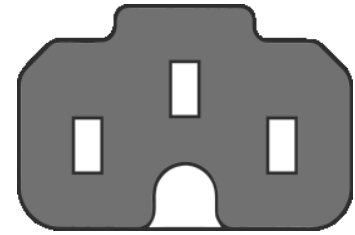
Dia 7.4.7 CEE 22 one notch and bulge
